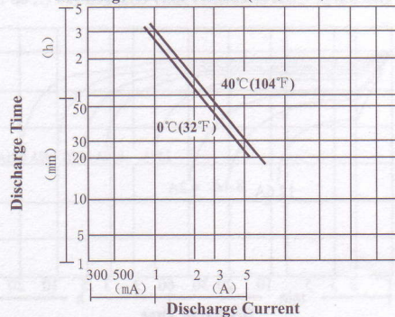
Discharge Characteristics (0°C/32°F, 40°C/104°F)
